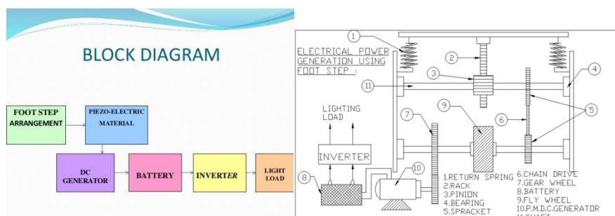
Fig.2. (a) Block diagram (b) Circuit diagram
